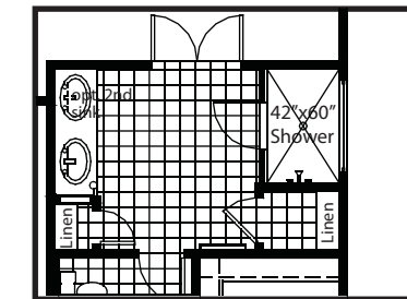
Optional 42"x60" Shower at Master Bathroom
