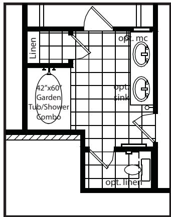
Optional Garden Tub/ Shower Combination at Master Bathroom
